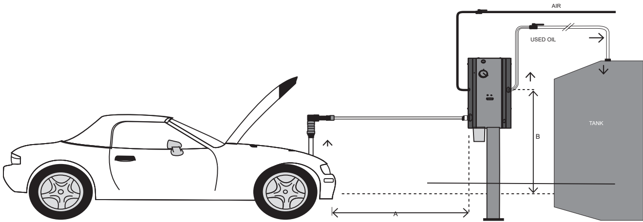
TYPICAL INSTALLATION Maximum installation distances: A: Maximum distance 20' (6 m). B: Maximum height between pump inlet and engine oil sump level, 3' (1 m).
